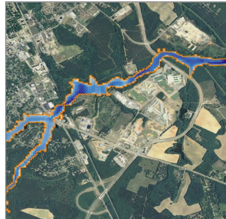
Figure 4. DCA can generate flood depth grids to illustrate the potential extent of flooding in a community
