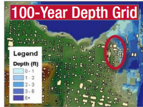
Figure 1. Example of Use of Depth Grids in Floodplain Mapping (not Johnson County)
