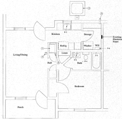
FLOOR PLAN - UNIT TYPE 1 SCALE 1/4" = 1'-0"
