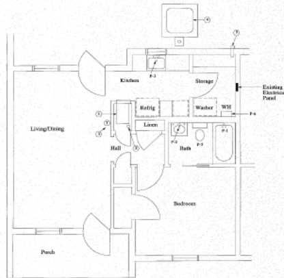
FLOOR PLAN - UNIT TYPE 2 SCALE 1/4" = 1'-0"
