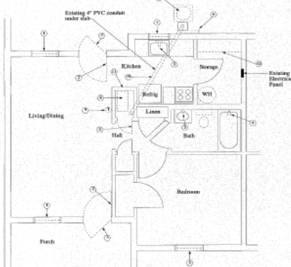
FLOOR PLAN - UNIT TYPE 1 SCALE 1/8" = 1'-0"
